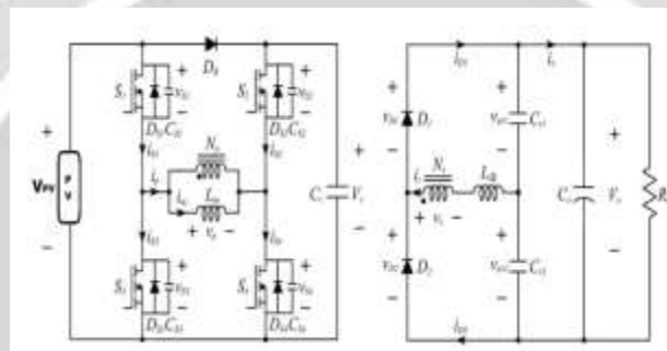
Fig-2: Circuit diagram of the proposed hybrid-type full-bridge dc/dc converter.
