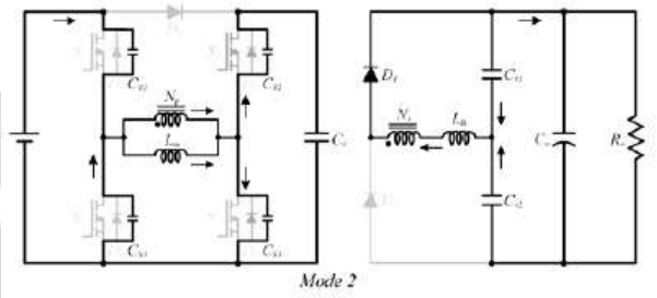
Fig-9: active clamp step up converter at mode2
