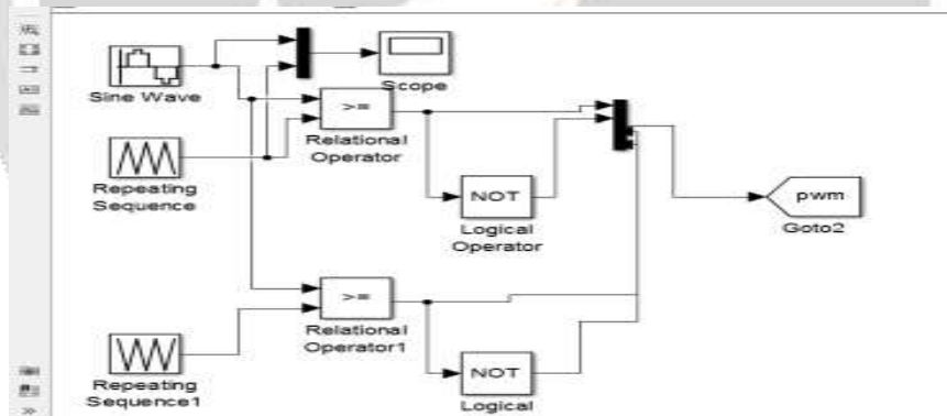
Fig-20: PWM technique
