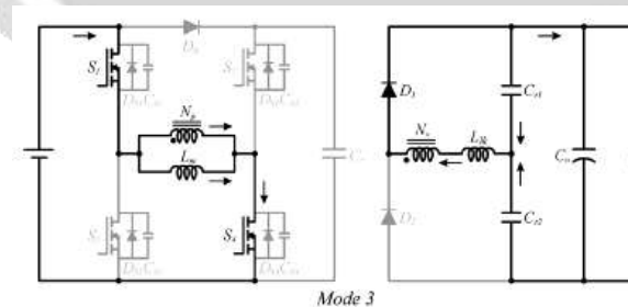
Fig-5: PSFB resonant converter at mode 3
