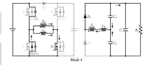
Fig-6: PSFB resonant converter at mode4
