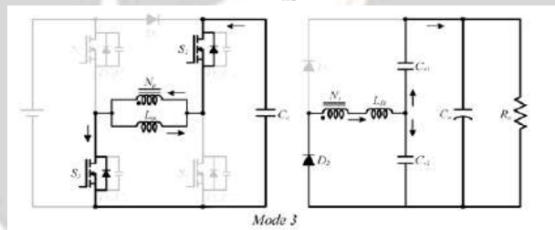
Fig-10: active clamp step up converter at mode3
