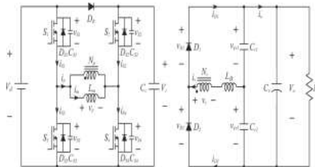
Fig-1: Circuit diagram of the hybrid-type full-bridge dc/dc converter.
