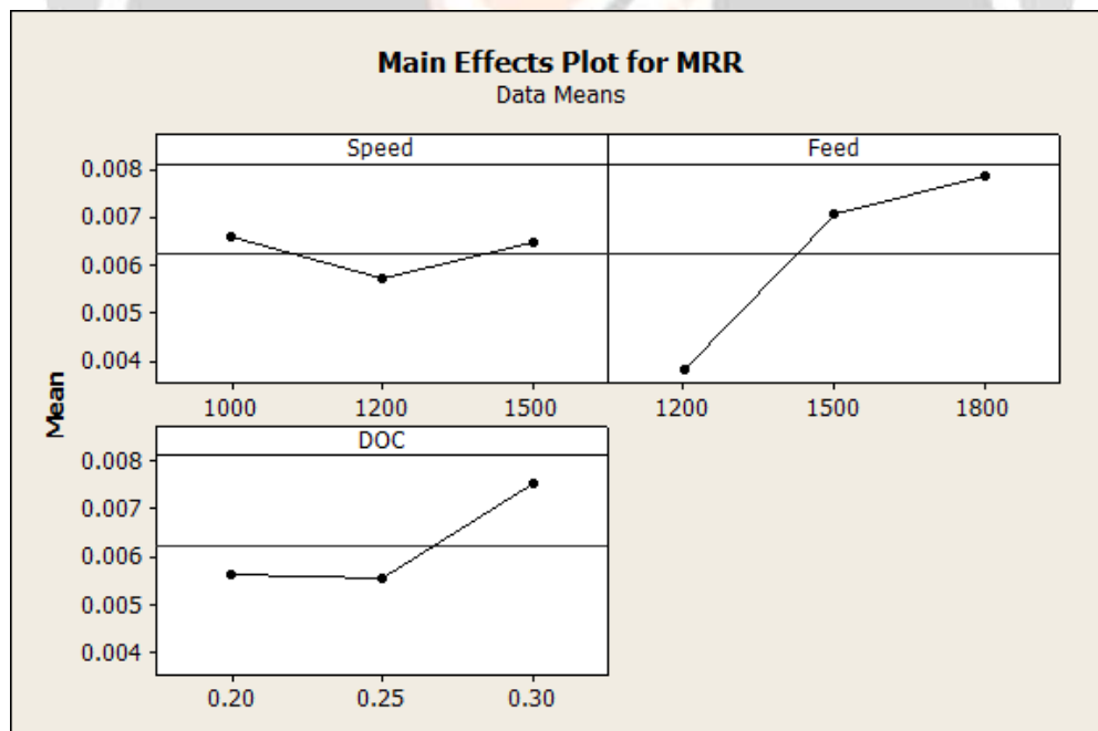
Fig 5.2 Main effect plot for MRR
