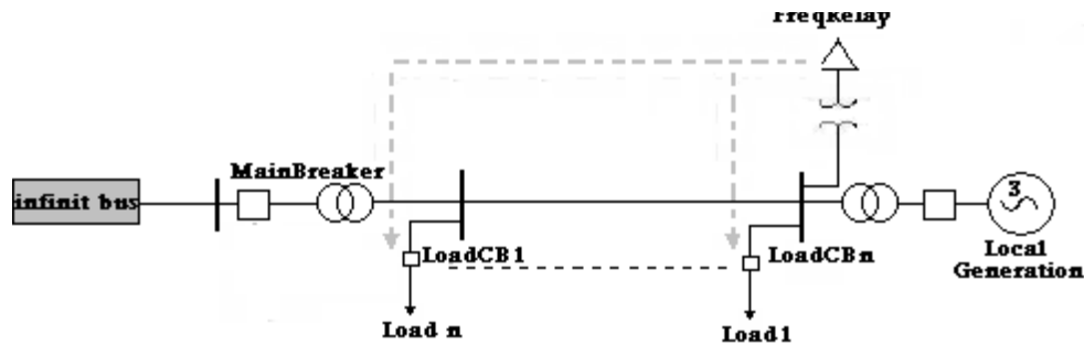
FIG. 2. UNDER FREQUENCY LOAD SHEDDING SCHEME
