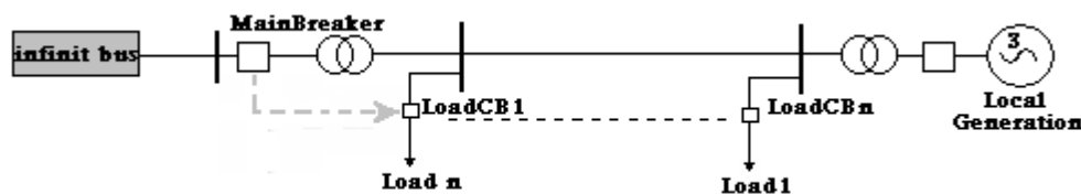
FIG. 1. BREAKER INTERLOCK LOAD SHEDDING SCHEME
