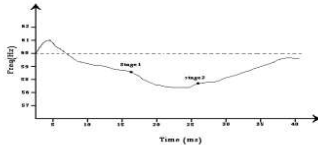
FIG. 3. SYSTEM FREQUENCY IN UNDER FREQUENCY LOAD SHEDDING
