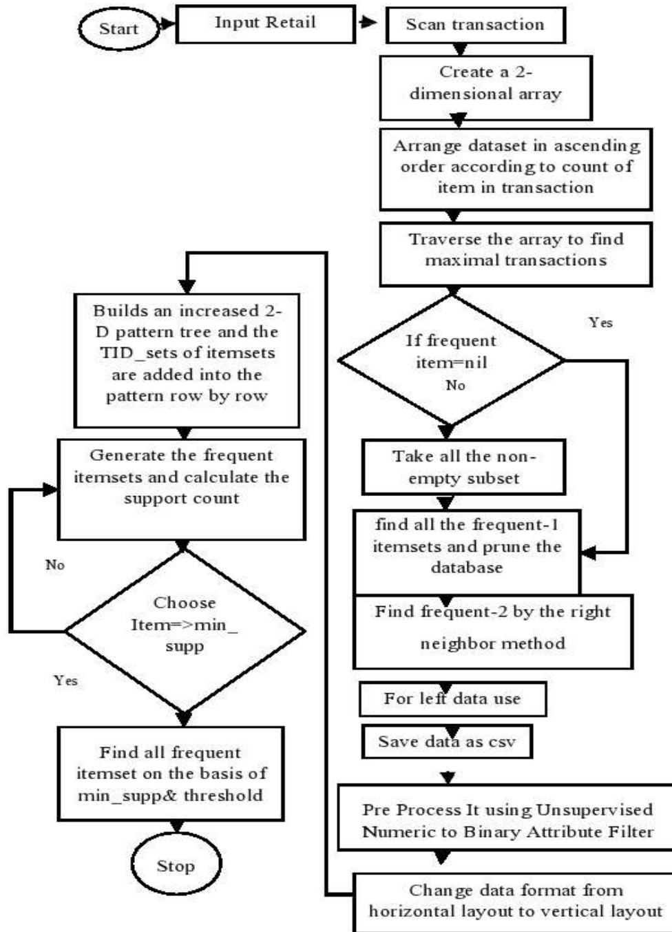
Fig. 3.1: Flowchart of Proposed Work
