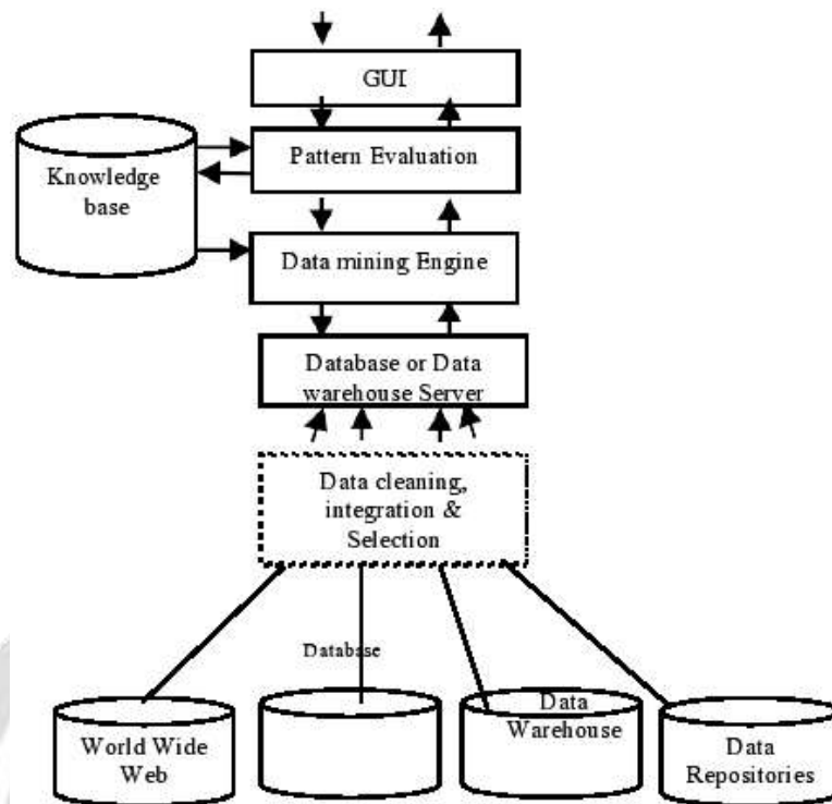
Fig. 1:Data Mining Architecture
