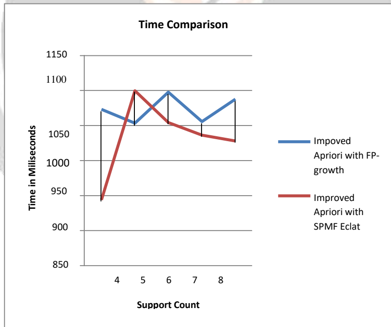
Fig 4.10: Elapsed time comparison
