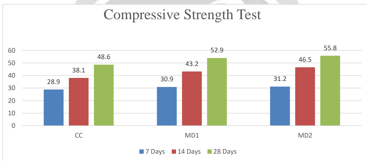
Fig 1. Compressive Strength Test
