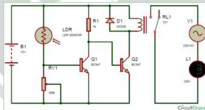
Figure 3 Automatic street light using LDR
