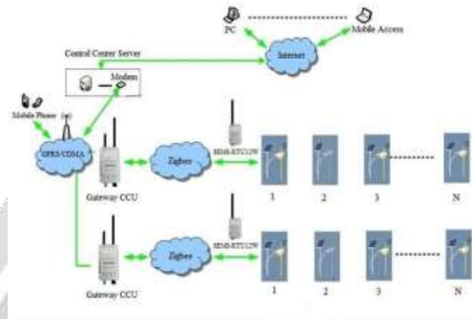
Figure 2 Control system for solar street lights
