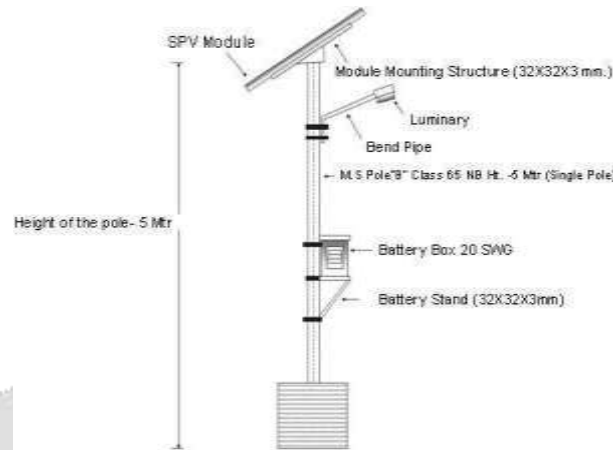
Figure 4 Solar panels
