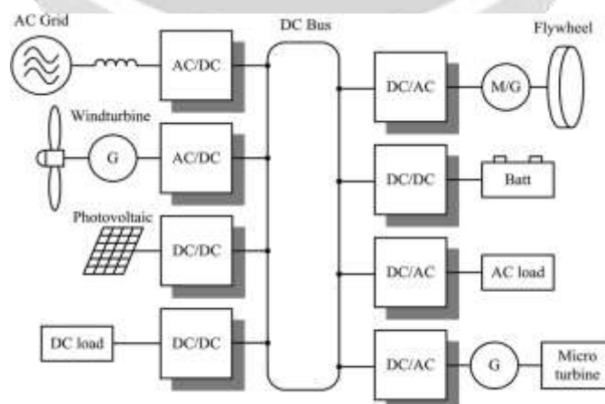
Fig. 1. Conceptual diagram of a dc-bus micro grid system.
