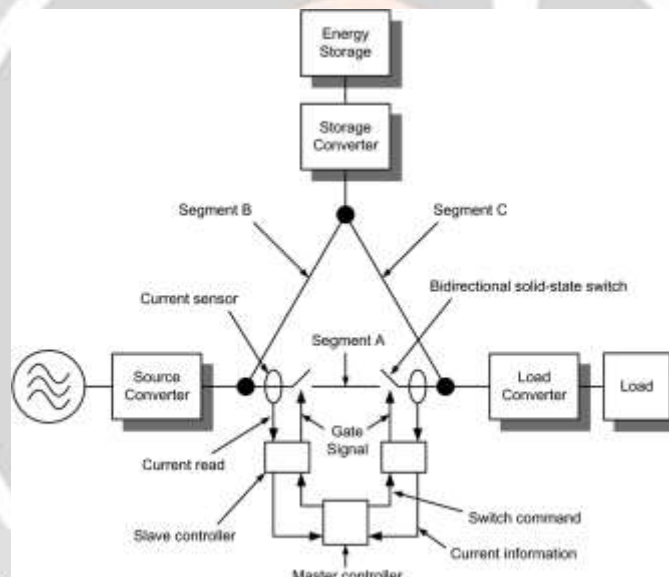
Fig. 2 Conceptual diagram of the proposed protection scheme. Protection controllers in segment B and C are omitted.
