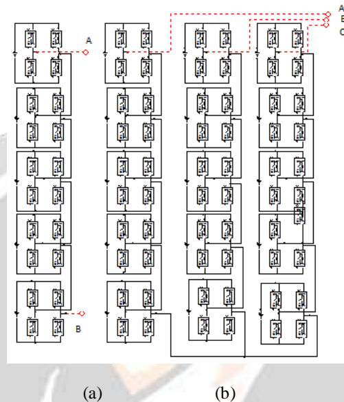
Fig: 1. Cascaded H-Bridge multilevel inverter for 11-level (a) per single phase (b) per three phase
