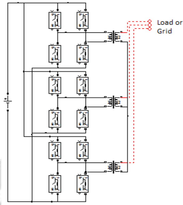
Fig: 2. Topology of H-Bridge cascaded transformer (HBCT) multilevel inverter
