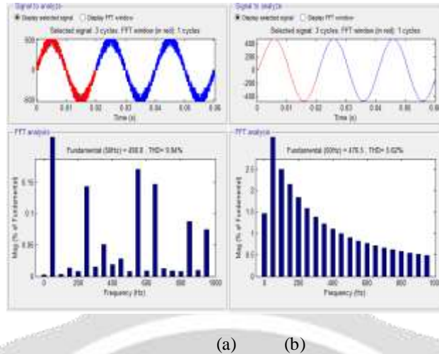
Fig: 7. Output waveforms of the HBCT multilevel inverter (a) without filter (b) with filter
