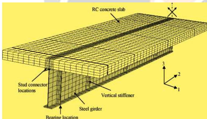
Fig. 1.1: Straight Composite Girder
