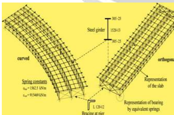
Fig. 1.2 : Curve Composite girder
