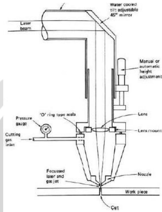
Figure 1: Laser cutting Process Setup
