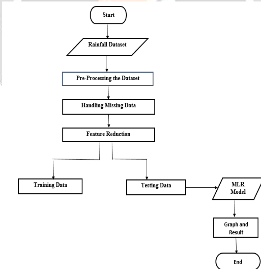
Fig-1: Rainfall Prediction Model
