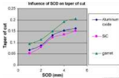
Fig. 3.4 Influence of SOD
