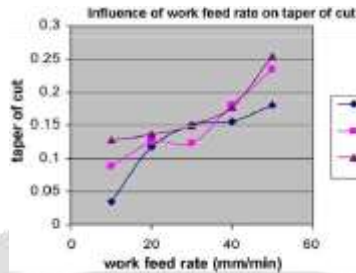
Fig. 3.5 Influence of feed rate on taper of cut
