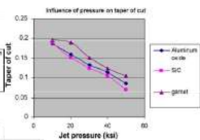
Fig. 3.6 Effect of pressure on taper of cut
