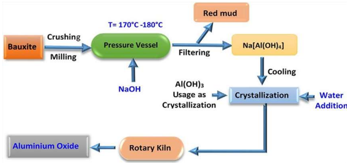
Fig-1: Bayer process of red mud and alumina production.
