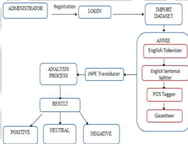
Fig -2: Block Diagram of Sentiment Analysis
