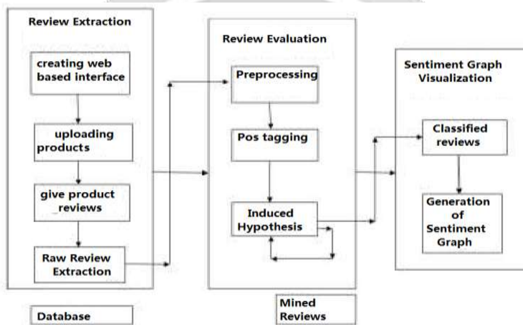
Fig -3: Proposed System Sentiment Analysis
