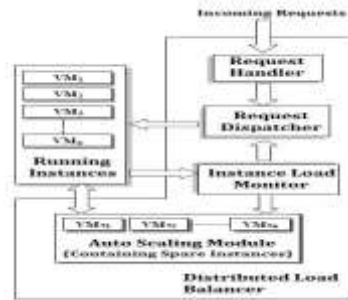
Fig 7 : distributed load balancer architecture. [1]
