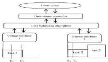
Fig 4. Probable states of allocation minimize waiting time. [3]
