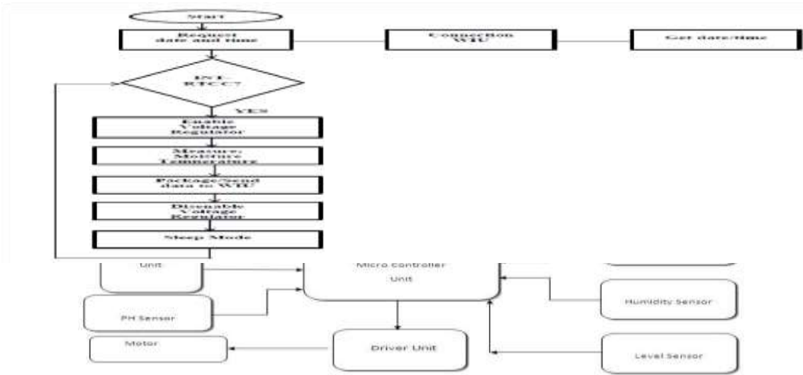
Fig.3. Flowchart of wireless sensor unit (WSU) for monitoring the soil moisture and temperature
