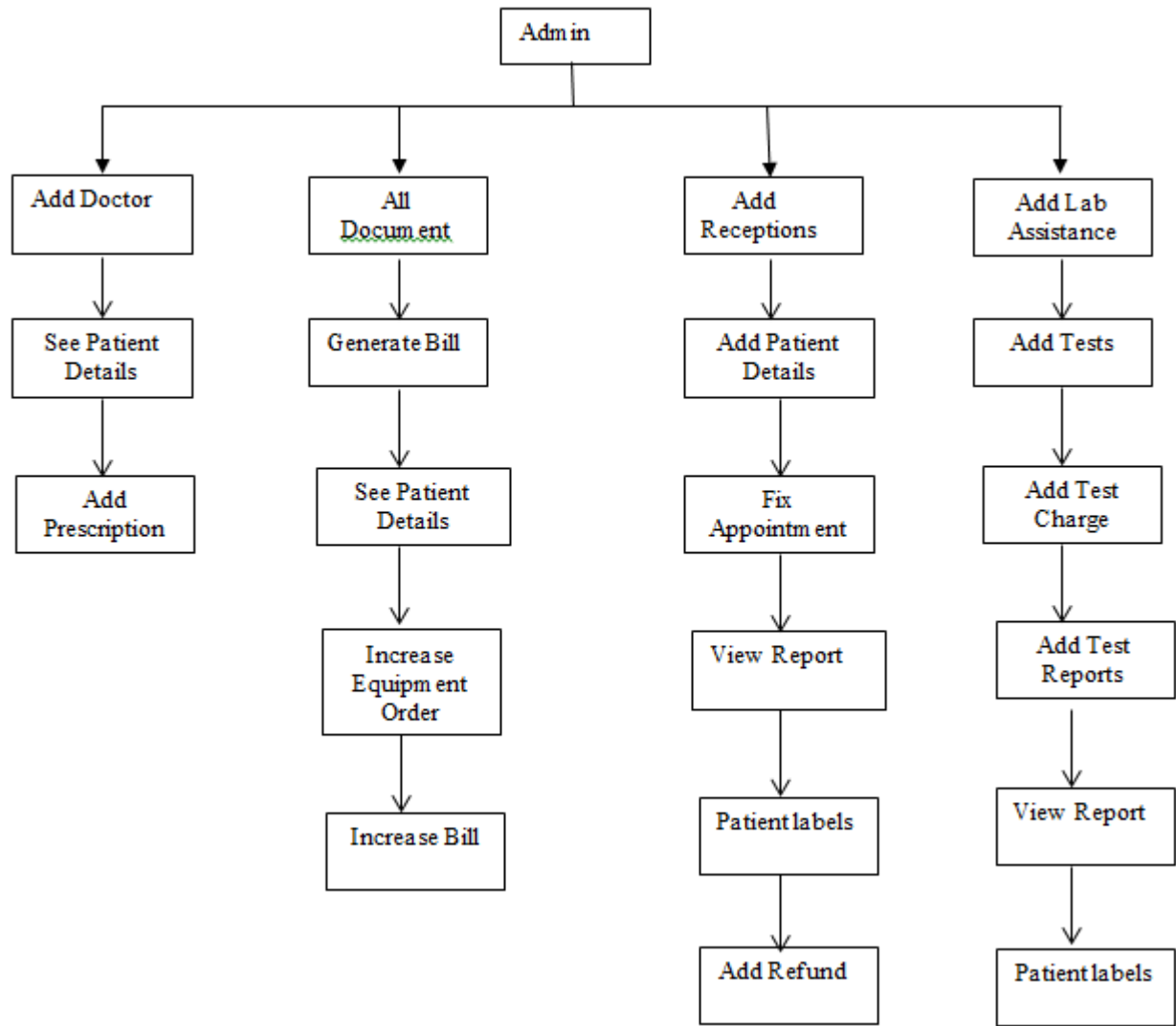
Fig 6.1. Deployment Diagram.
