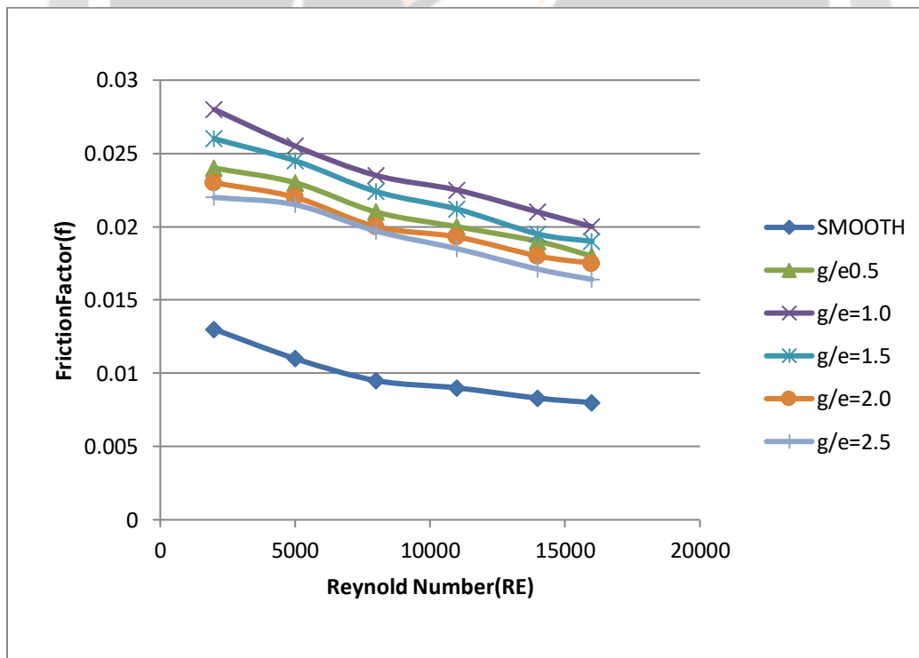
Fig. 6 Comparison between Friction factor and Reynolds number at different gap width ( g/e )
