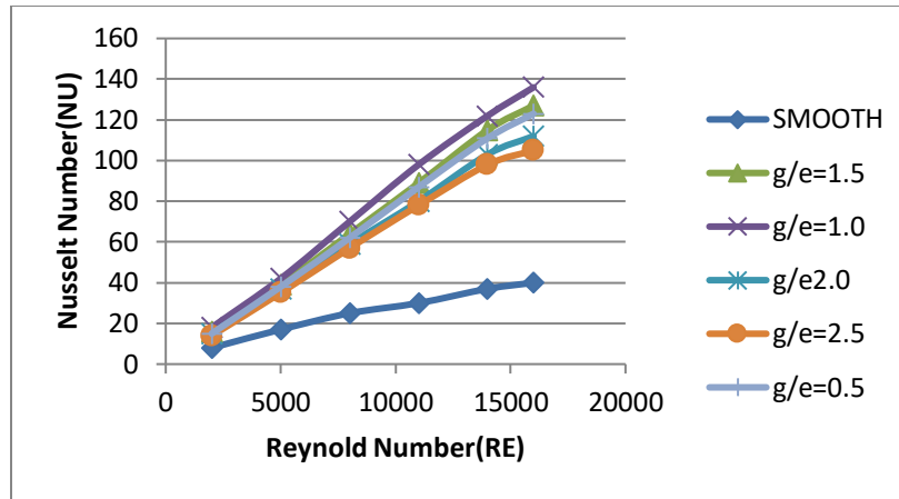
Fig. 4. Variation of Nusselt number with Reynolds number for different Values of relative gap width
