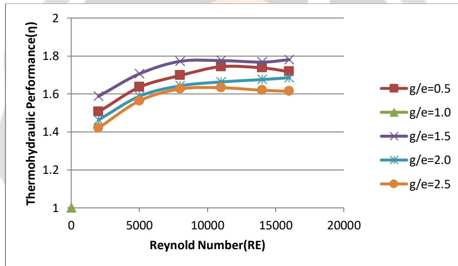
Fig.5 Thermo-hydraulic performance parameter as a function of Reynolds Number for different relative gap width ( g/e )
