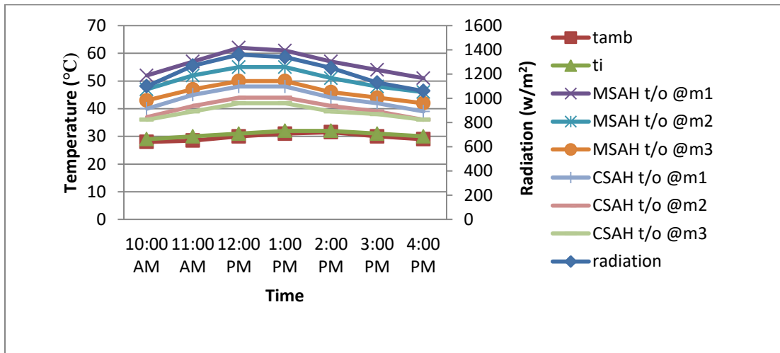
Graph 4.1 Comparative variation of temperature with time and radiation
