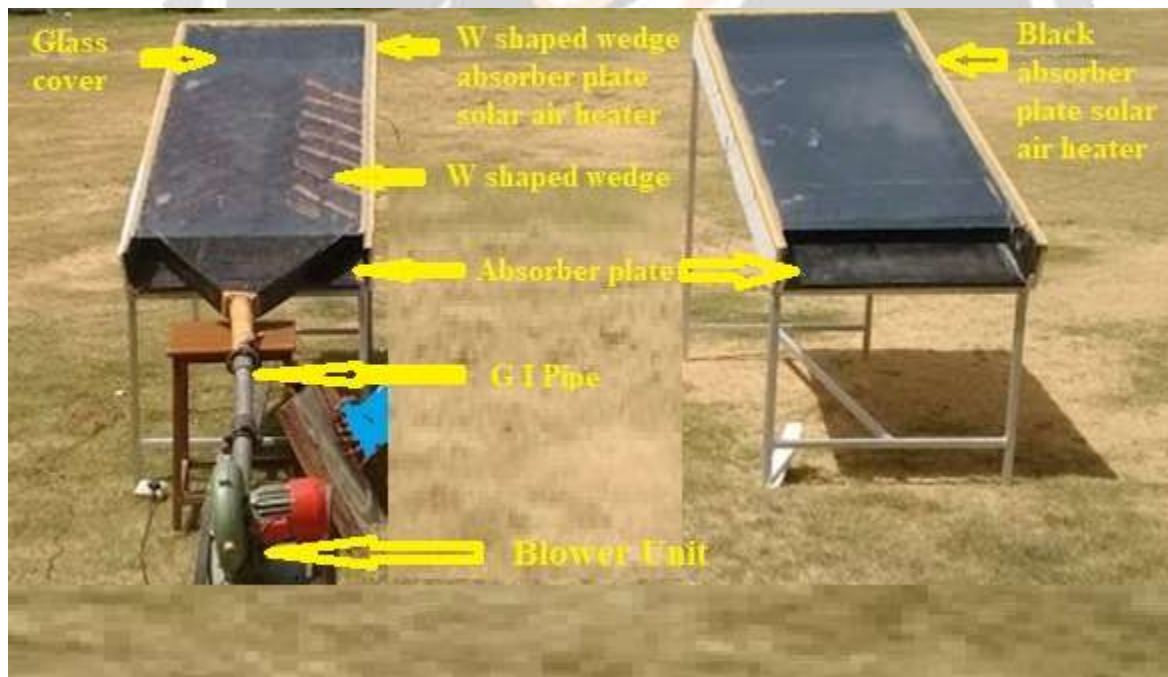
Figure 1. Pictorial view of experimental setup
