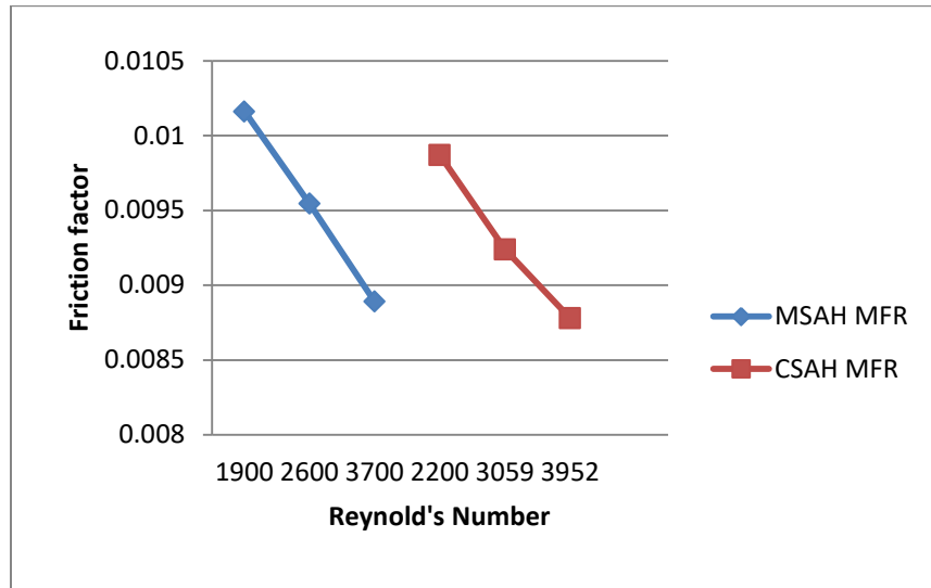
Graph 4.3 Comparative variation of friction factor with Reynolds number
