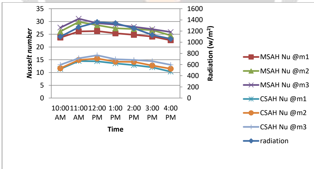
Graph 4.4 Comparative variation of Nusselt number with time
