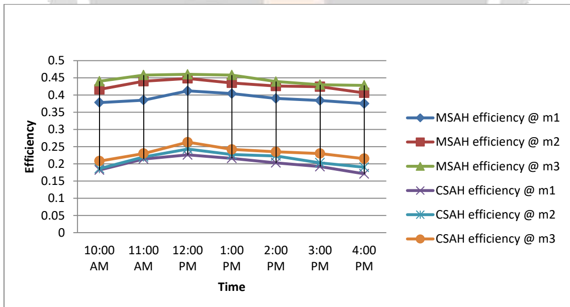
Graph 4.2 Comparative variation of thermal efficiency with time
