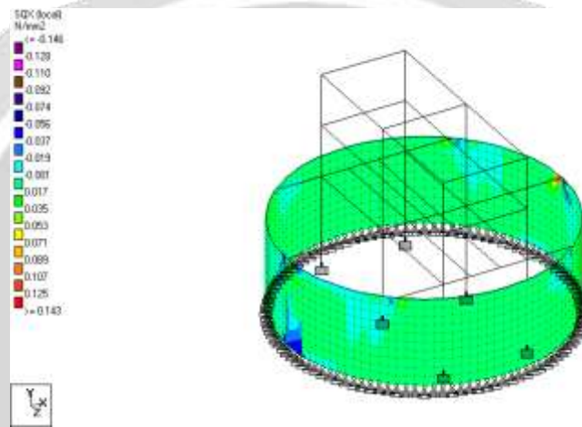
Fig 6: Design of base slab
