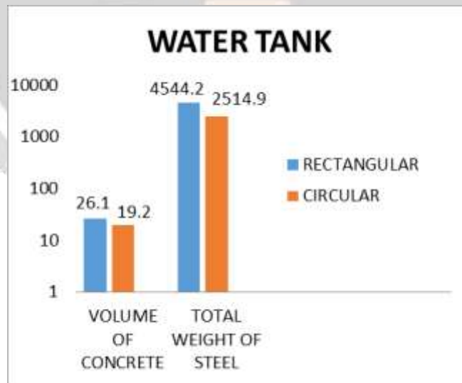
Fig 7: Water Tank
