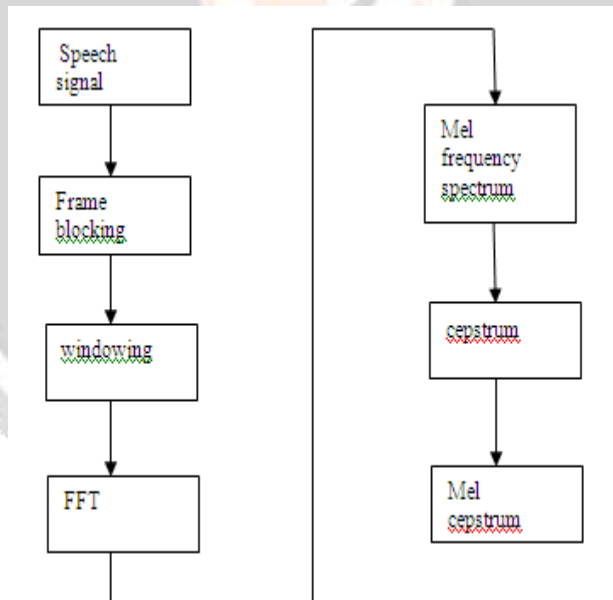
Fig -2: MFCC Block Diagram
