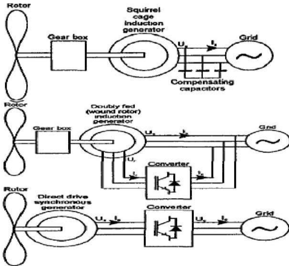
Fig2. Widely used contemporary wind turbine concepts
