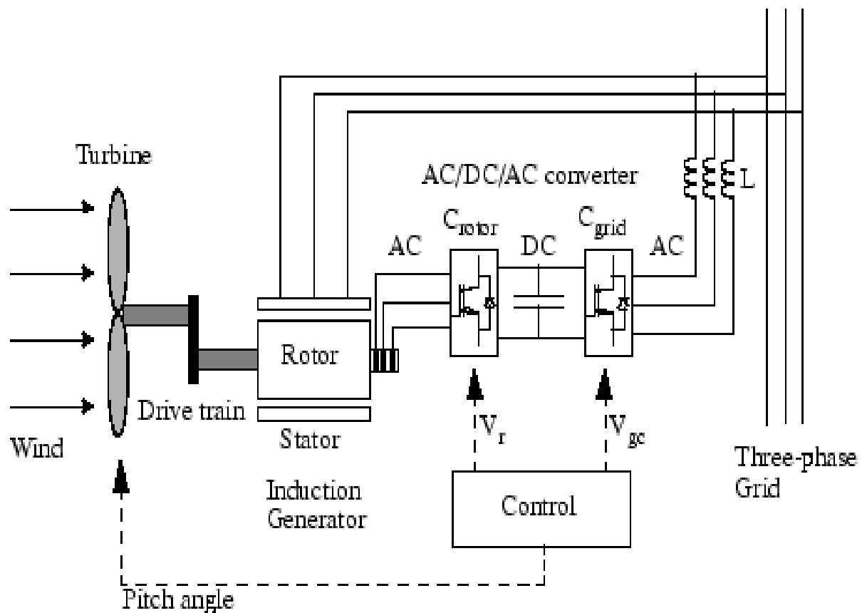
Fig1. DFIG model
