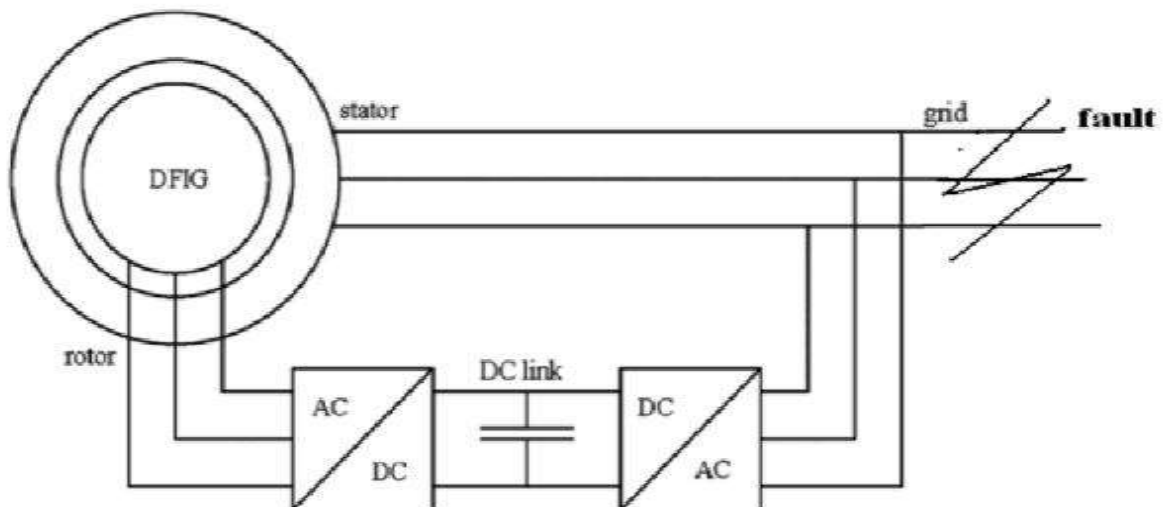
Fig3. Block diagram of DFIG with fault at grid side
