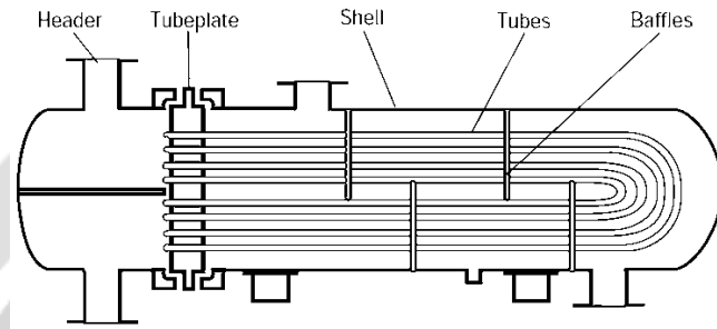
Figure 1.2 U-tube heat exchanger
