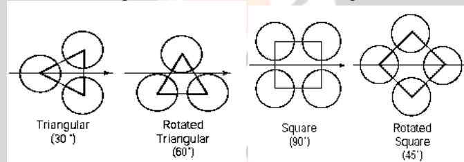
Figure 1.3 Tube Layout Angles
