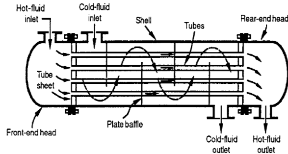
Figure 1.1 Shell-and-tube exchanger (BEM) with one shell pass and one tube pass or Fixed-tube sheet heat exchanger.
