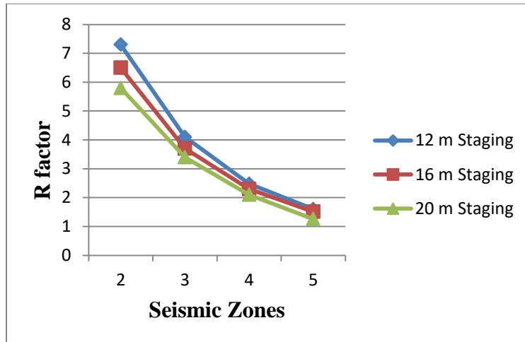
Fig 3.2.1: R factor v/s seismic zones for different staging of Empty water tank
