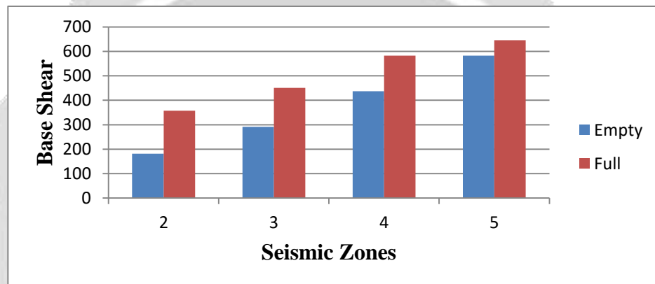
Fig 2.2: Base shear v/s seismic zones for different Tank condition
