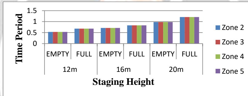
Fig 3.1: Time period v/s Different Staging for different zones and tank condition of water tank
