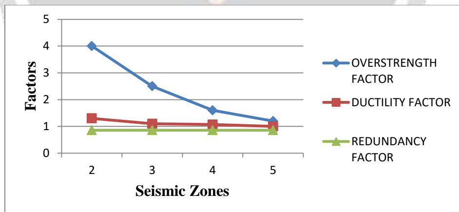
Fig 2.21: Factor's v/s seismic zones for Empty water tank.
