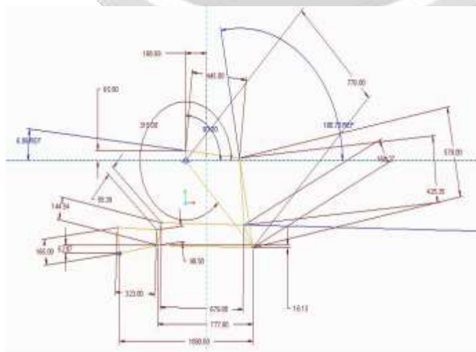
Position, velocity and acceleration analysis for crank-rocker
