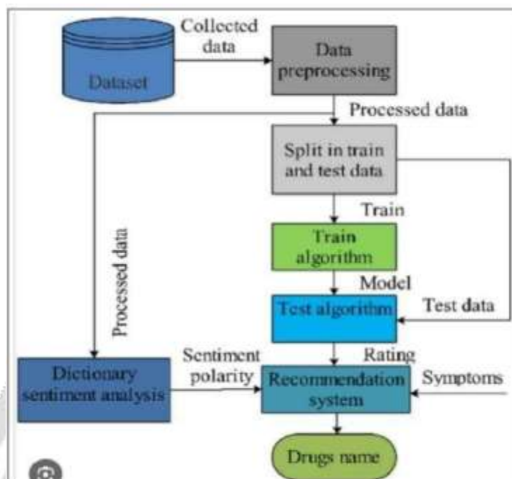
Fig 1: Flowchart of Recommendation System
