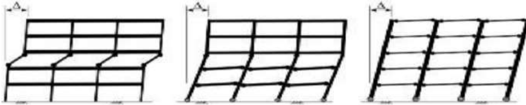
Fig: 4: Story mechanism Intermediate mechanism Beam mechanism (Reference: Moehle et ai., 2008)
