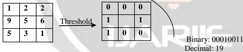
Fig 4: Example calculation of LBP
