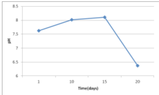
Figure 2. pH variation in sewage irrigated soil.
