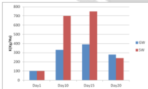
Figure 4. Potassium (K) variation with time.
