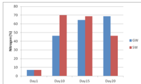
Figure 6. Variation of Nitrogen with time.
