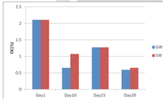
Figure 3. Organic Carbon variation with time.
