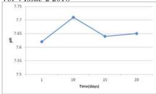
Figure 1. pH variation in groundwater irrigated soil.
