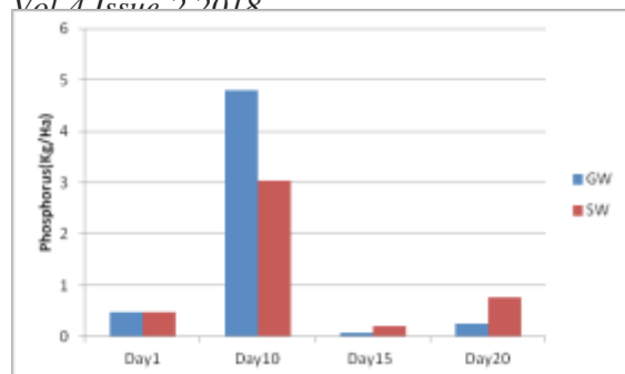
Figure 5. Phosphorus (P) variation with time.
