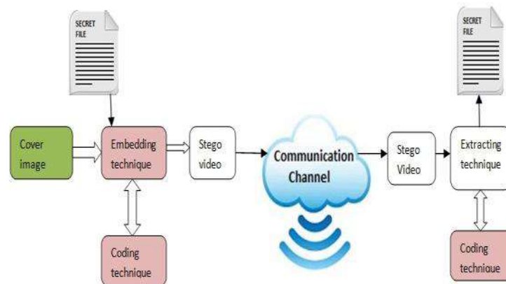
Fig -1: structure of Steganography system [6]
