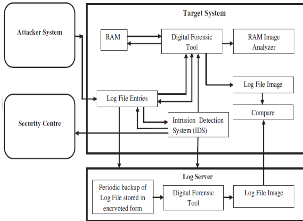
Figure 1: Automated Digital Forensic Technique with Intrusion Detection System Log Server
