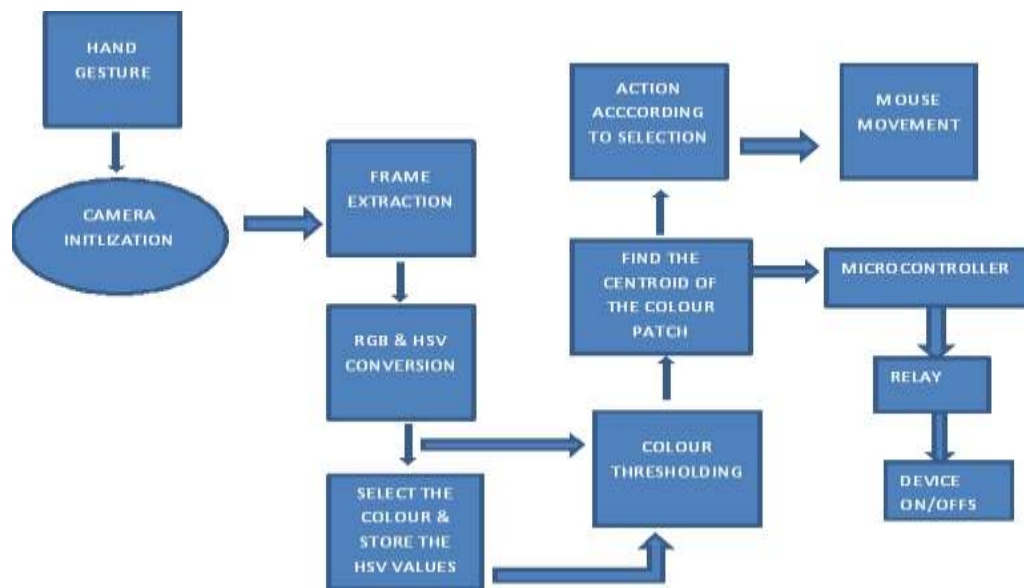
Figure 3:- System Flow
