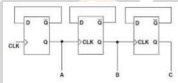
Figure 1: 3-bit Down Ripple Counter
