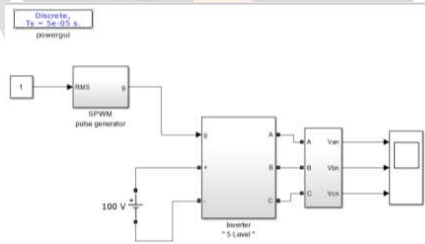
Fig-5: Proposed circuit using MATLAB design
