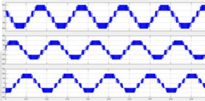
Fig-13: The Output phase voltage for CSVPWM
