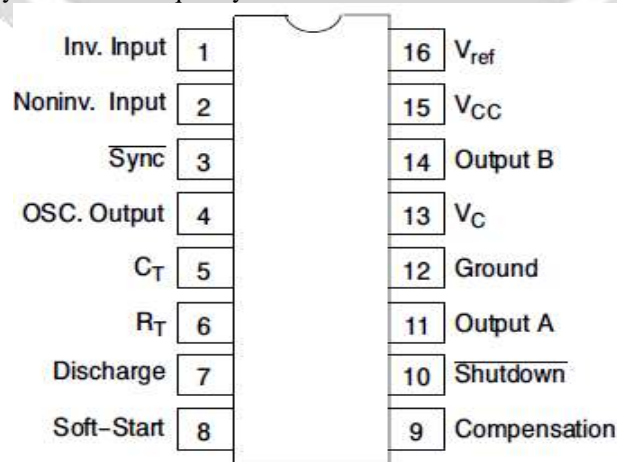
Fig -1: Pin diagram of IC SG 3525
