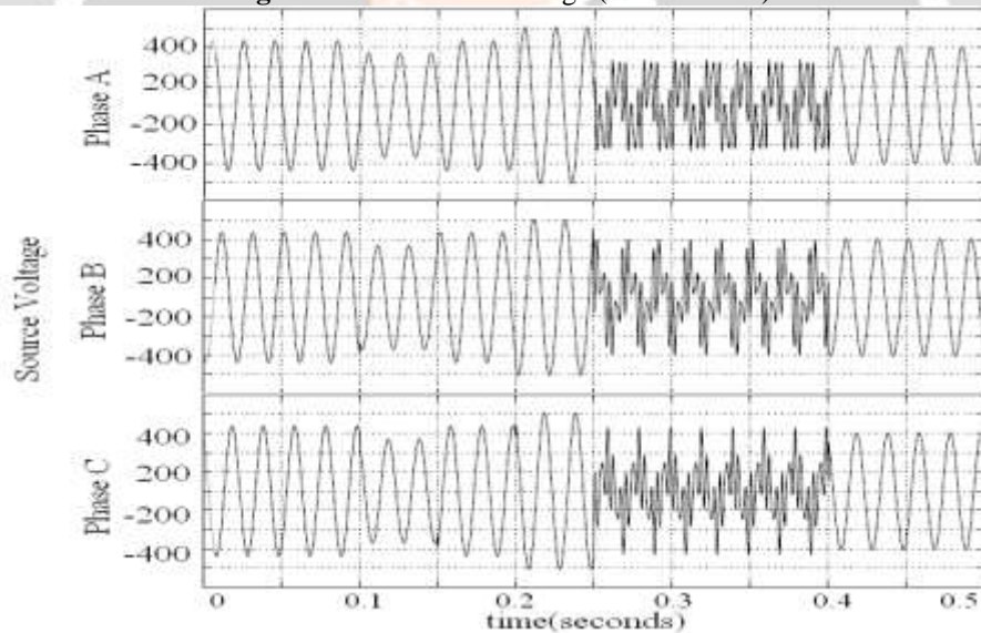
Fig-9: Source Voltages per phase
