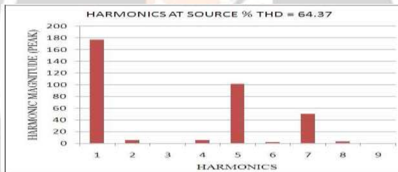
Fig-11: Source voltage harmonic spectrum
