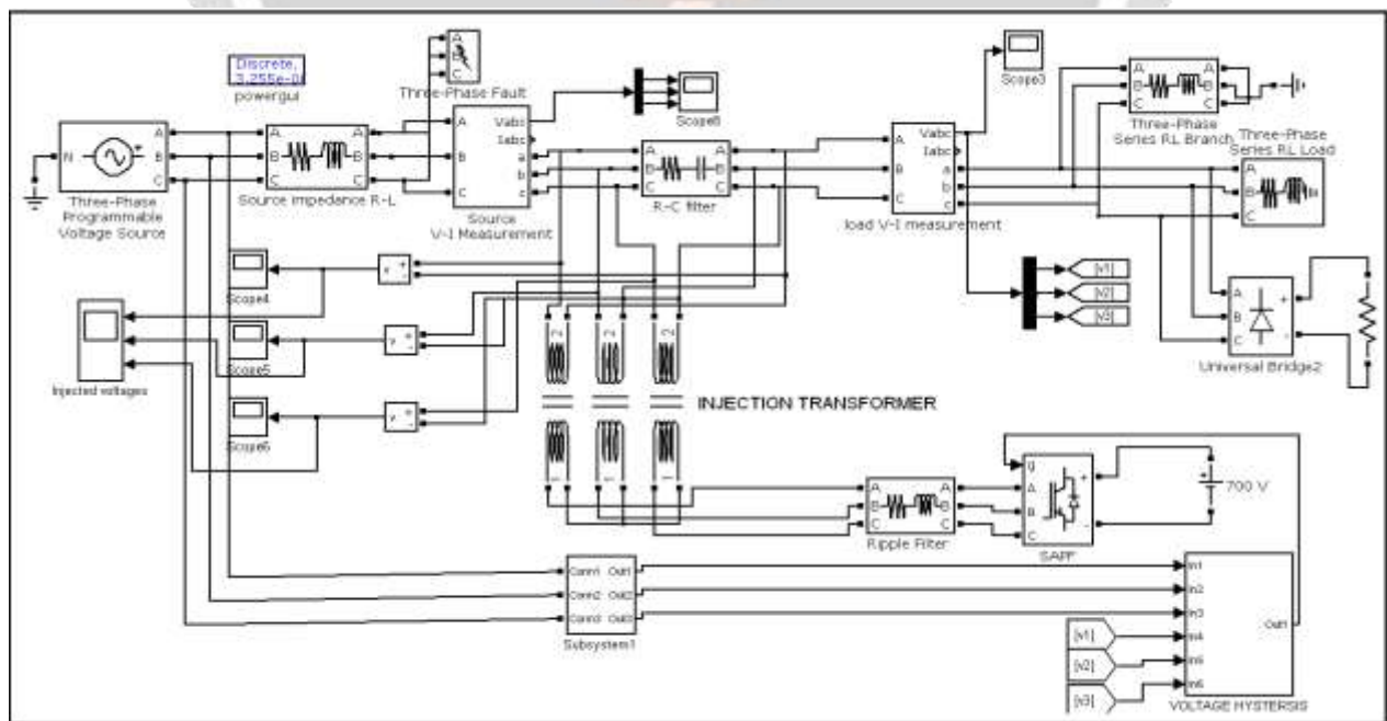
Fig -1: MATLAB simulation model of proposed Voltage stabilizer using series active power filter
