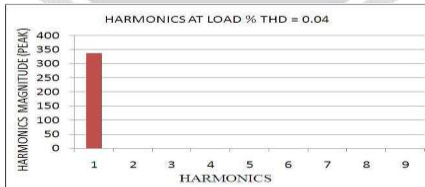
Fig-7: Load voltage harmonic spectrum
