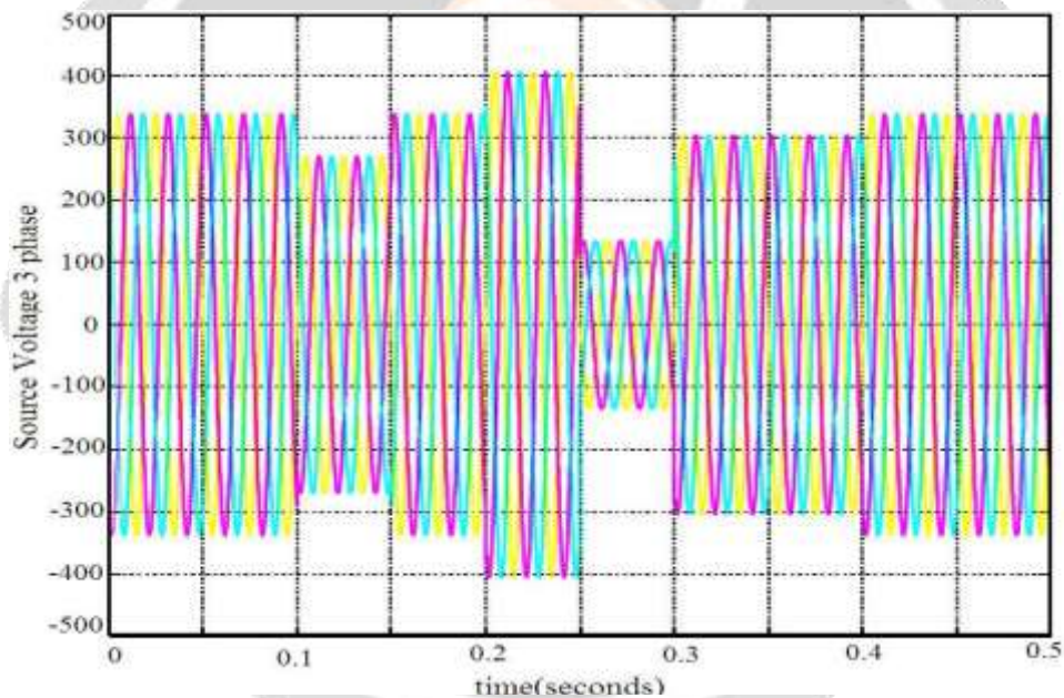
Fig -2: 3-Phase Source voltage (Line-Ground)
