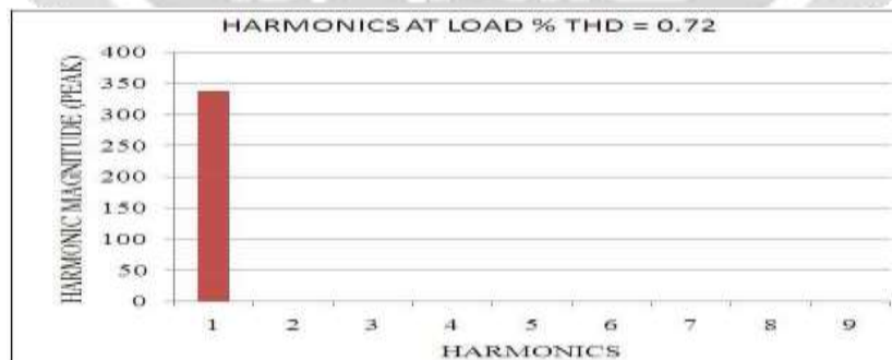
Fig-12: Load voltage harmonic spectrum
