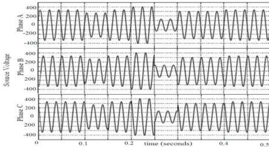
Fig-3: Source Voltage in each Phase
