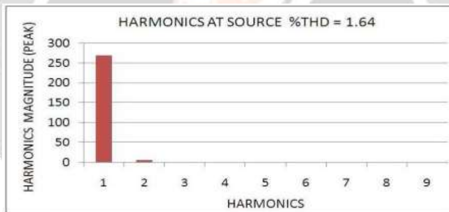
Fig-6: Source voltage harmonic spectrum
