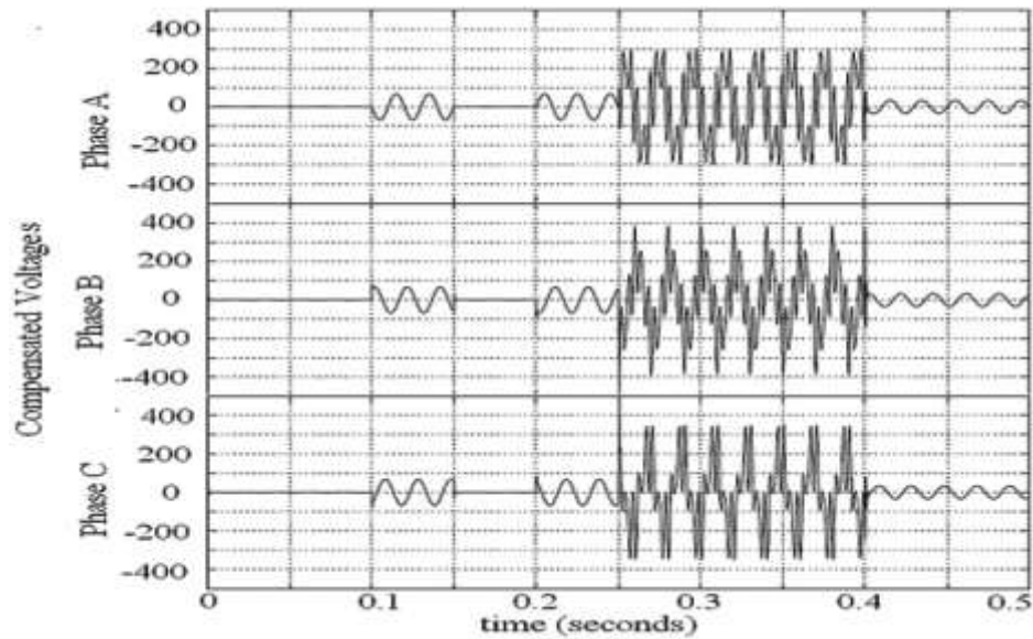
Fig-10: Compensated voltages injected for each phases
