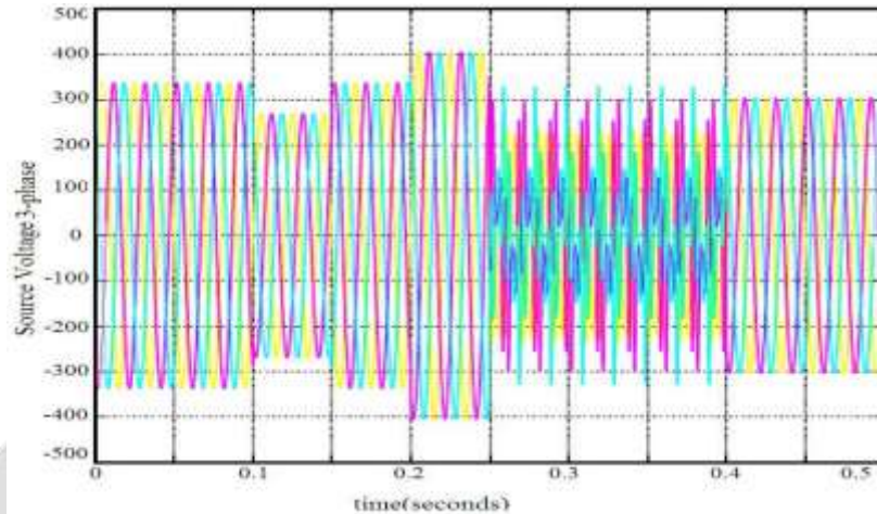
Fig-8: 3-Phase Source voltage (Line-Ground)
