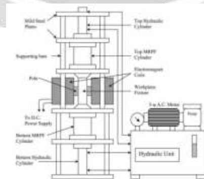
Fig. 1.5 Schematic diagram of the MRAFF setup
