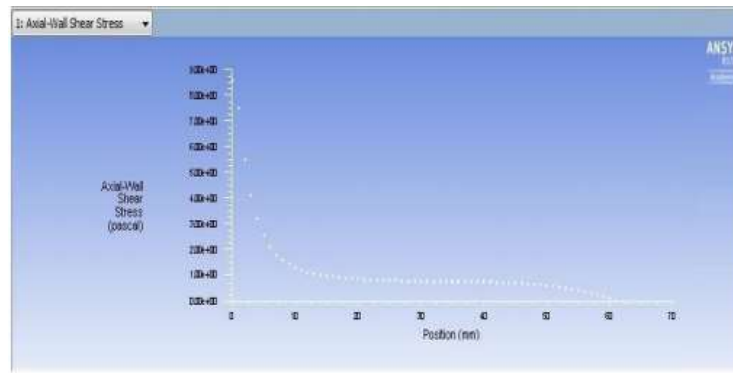
Fig. 3.7 Axial wall shear stress with position
