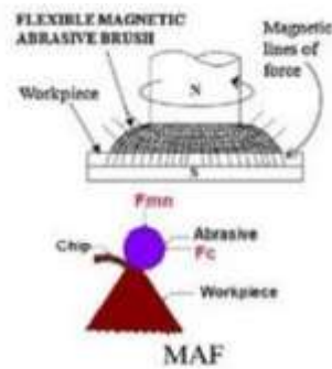
Fig. 1.1 Magnetic abrasive flow machining
