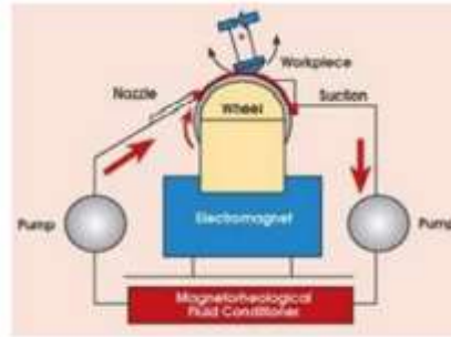
Fig. 1.3 Magneto rheological flow polishing
