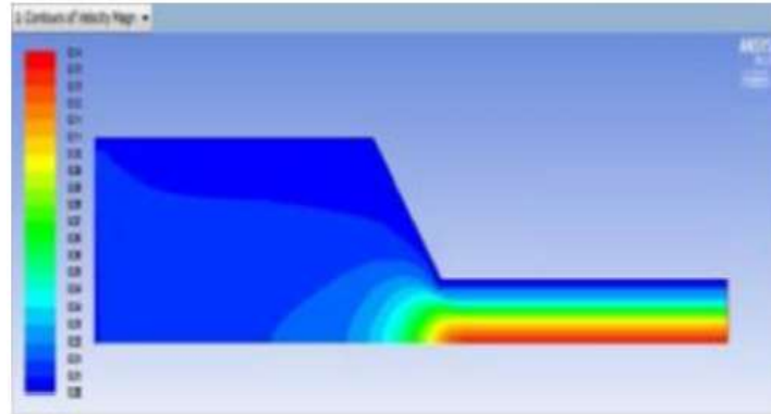
Fig. 3.1 Velocity distribution along the workpiece fixture
