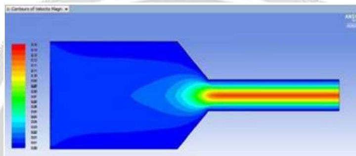
Fig. 3.2 Velocity distribution on full view of work piece fixture
