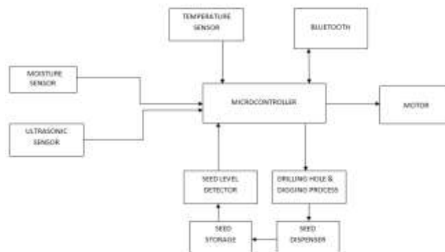
Fig: Block diagram of robot
