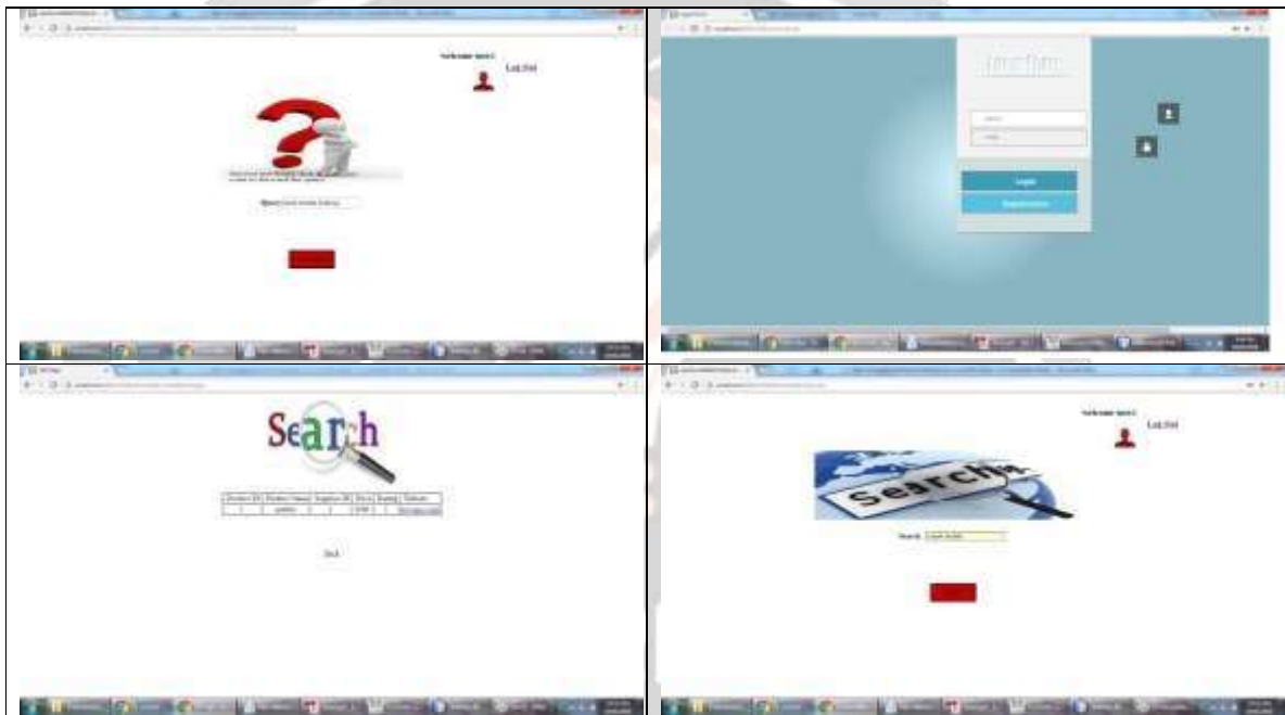
Figure 9: User implementation
