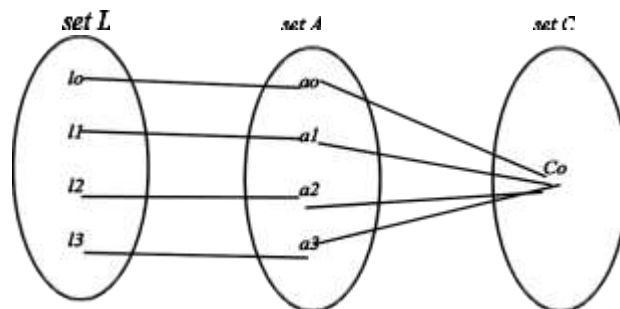
Figure 2: vein diagram 1
