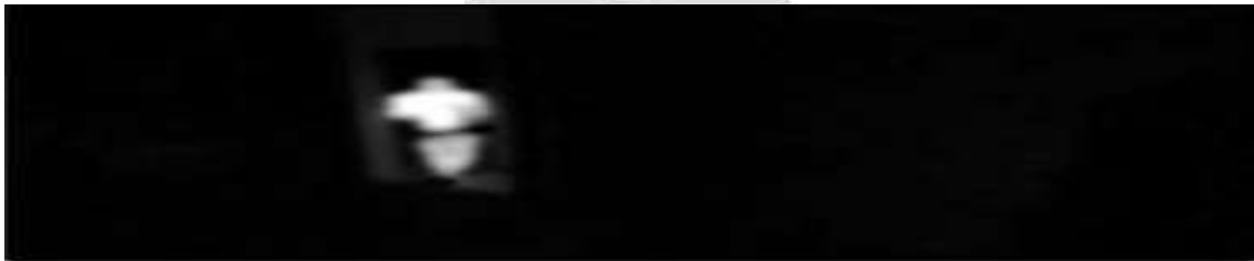
Figure 5: Background detection
