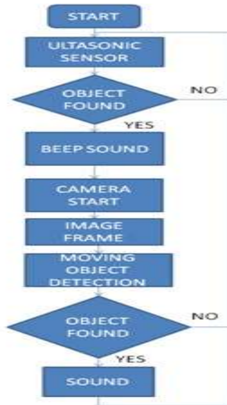
Figure 2: Flow Diagram of Proposed Algorithm
