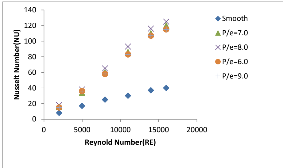
Fig. 4. Variation of Nusselt number with Reynolds number for different Values of combination of relative roughness pitch(P/e)
