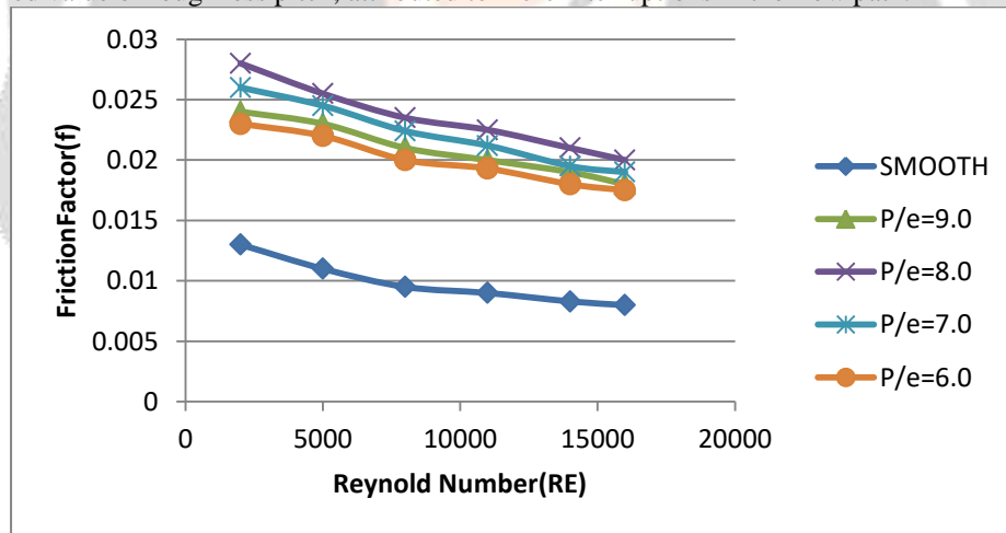
Fig. 6 Comparison between Friction factor and Reynolds number at different roughness pitch(P/e)
