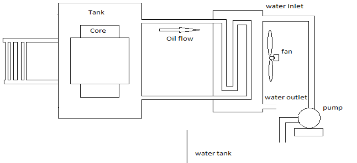
Fig.:2 The sketch of cooling system applied in transformer with ONWFAF.
