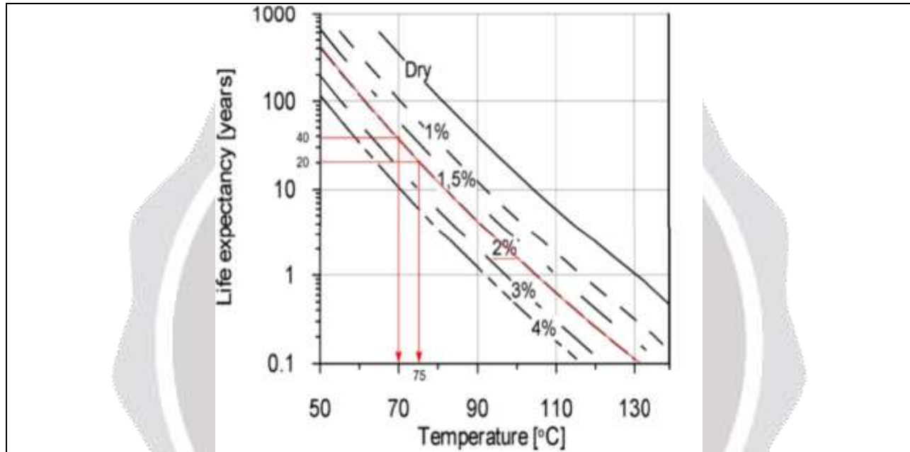
Fig-:1 Dependency on temperature and humidity in the life expectancy of paper insulation in transformer
