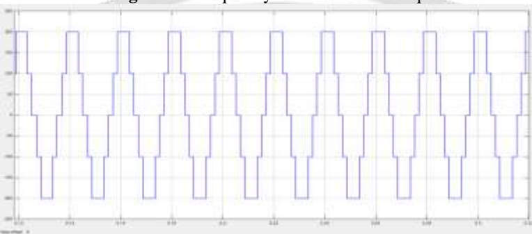
Fig-10: Five-level Output voltage of Inverter
