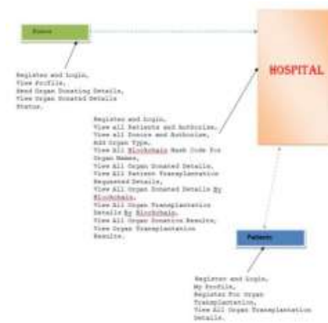
Fig. 1. Proposed Architecture
