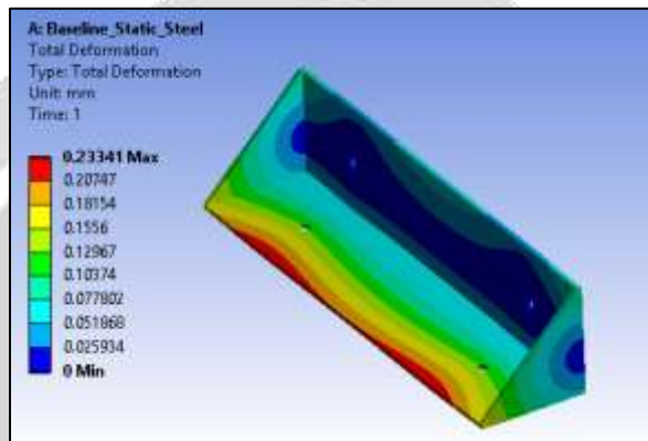
Fig.4.Total deformation plot for Steel AC mounting bracket 1
