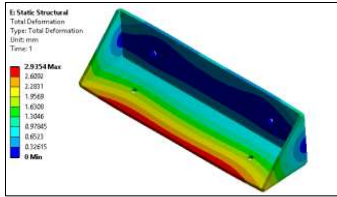
Fig.6.Total deformation plot for GFRP AC mounting bracket 1
