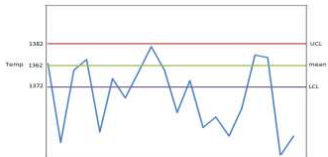
Fig 4: Control chart for Temperature
