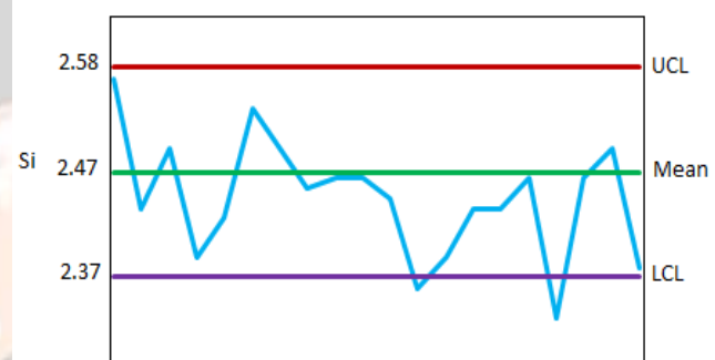
Fig 6: Control Chart For Silicon
