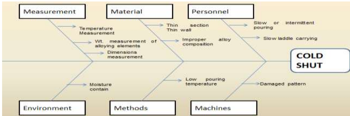
Fig 3: Ishikawa diagram
