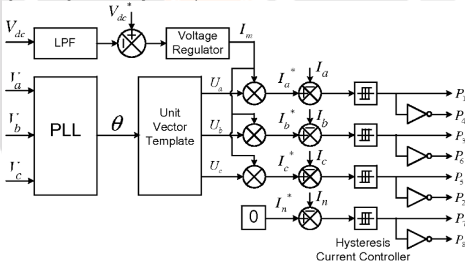
Fig: 3- Block diagram representation of grid-interfacing inverter control.
