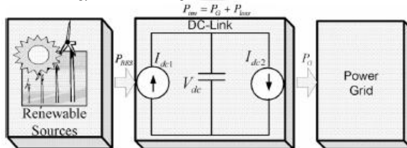
Fig: 2- DC-Link equivalent diagram.
