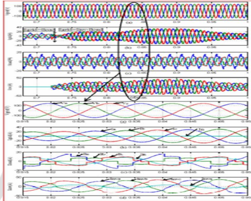
Fig: 4- simulation results: (a) Grid voltages; (b) Grid currents; (c) Unbalanced load currents; (d) Inverter Currents.
