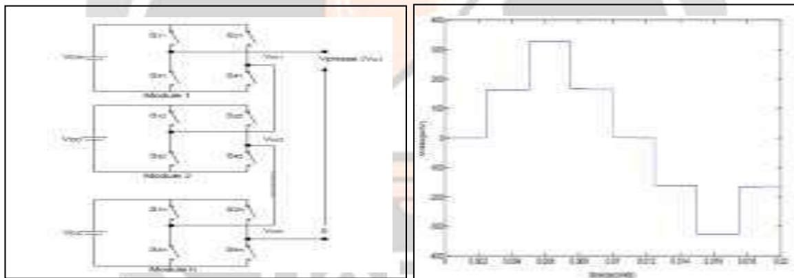
Fig. 2: Single phase 5-level Cascaded H-Bridge multilevel inverter with its output voltage waveform.
