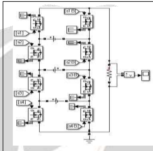
Figure 3: Single Phase CHBMLI
