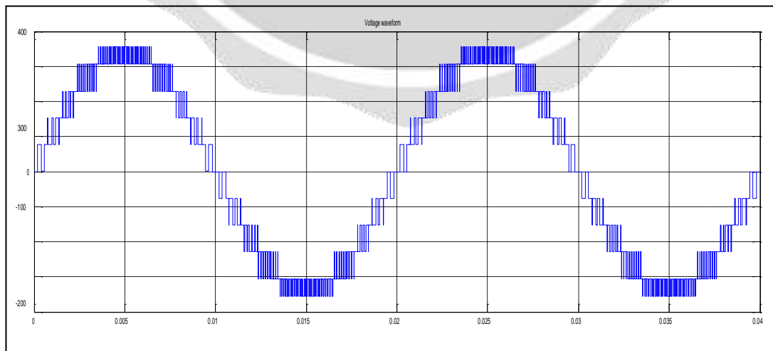
Fig. 6: Output voltage 11 level CHB-MLI for R Linear loading using VFPWM
