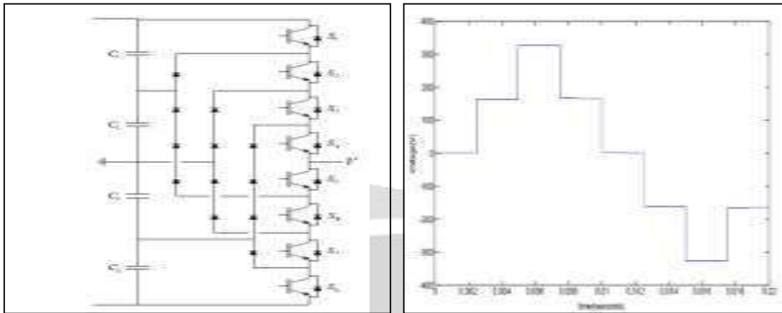
Fig. 1: Single phase 5-level Diode Clamped multilevel inverter with its output voltage waveform.
