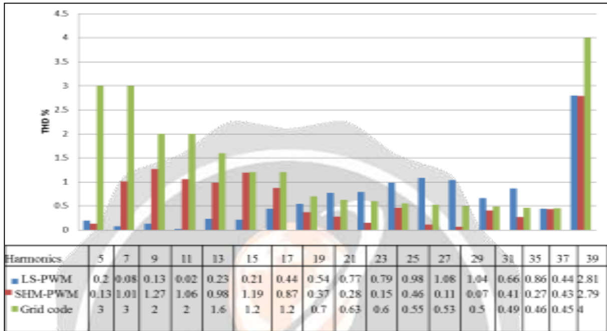
Figure 7: Output voltage harmonic comparison for 11 level CHB-MLI for linear loading using VF PWM
