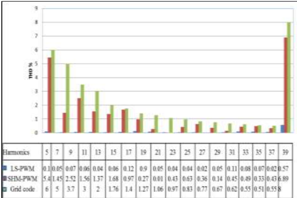
Fig. 5: Output voltage harmonic comparison for 11 level CHB-MLI for IPD PWM
