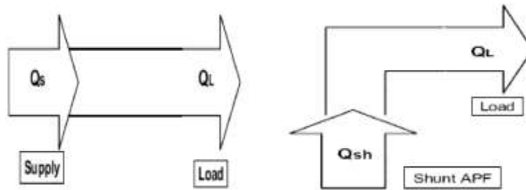
Fig-4: Reactive Power Flow No UPQC (b) Shunt APF ON
