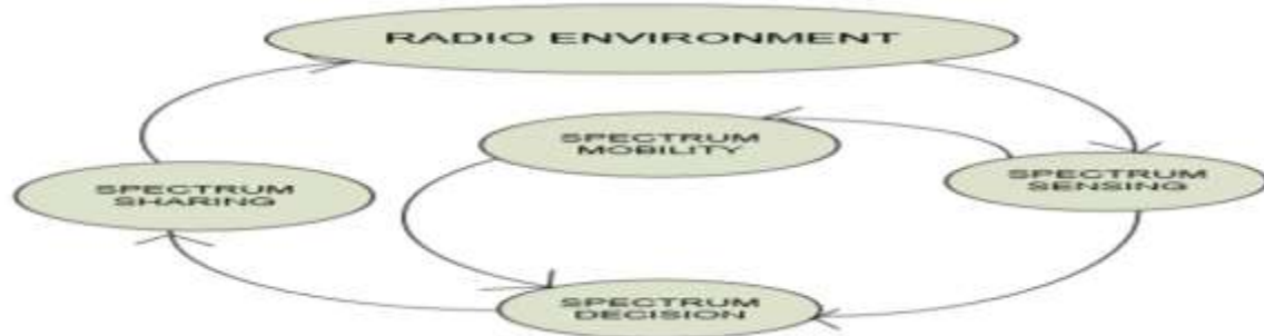
Fig 3: cognitive cycle[8]
