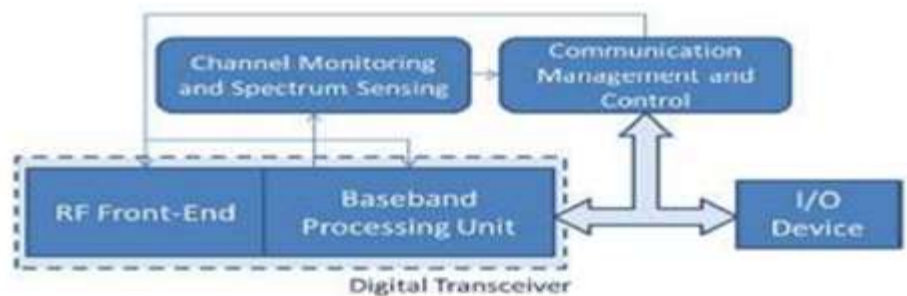
Fig 2: cognitive radio physical architecture.[8]
